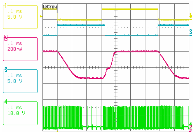
FIGURE 31. C4 ENTRY/EXIT, V_{IN} = 12.6V , I_o = 0.7A , HFM VID = 1.1V, LFM VID = 0.9V, C4 VID = 0.7625V, FDE = DPRSLPVR, Ch1: DPRSTP#, Ch2: Vo, Ch3: DPRSLPVR/FDE, Ch4: PHASE
