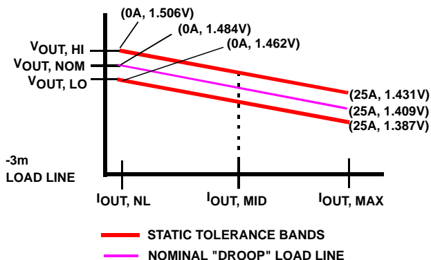
FIGURE 11. IMVP-IV™ ACTIVE MODE STATIC LOAD LINE
