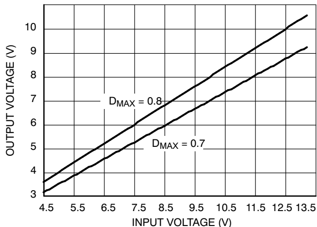
Figure 11. Maximum Input to Output Voltage
