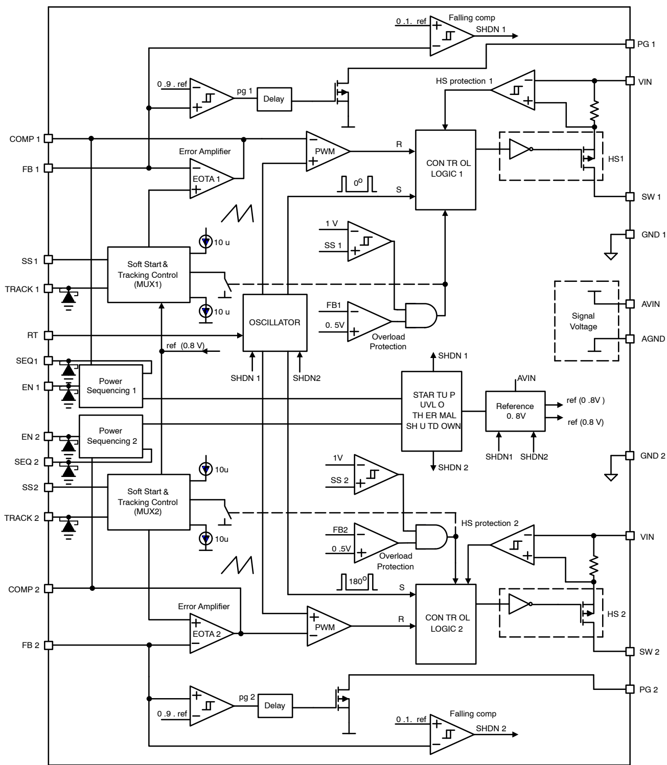
Figure 2. Block Diagram
