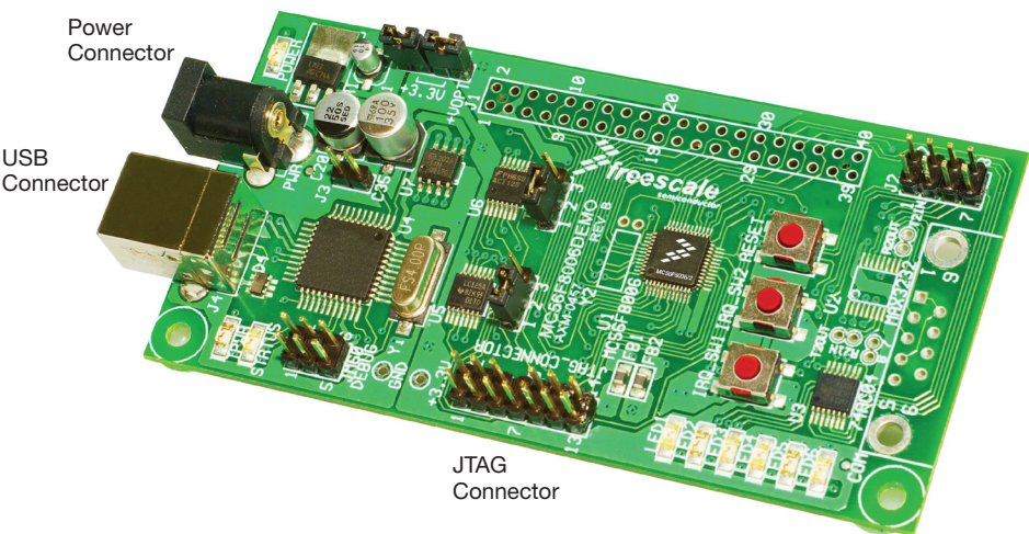
Figure 1. MC56F8006DEMO
