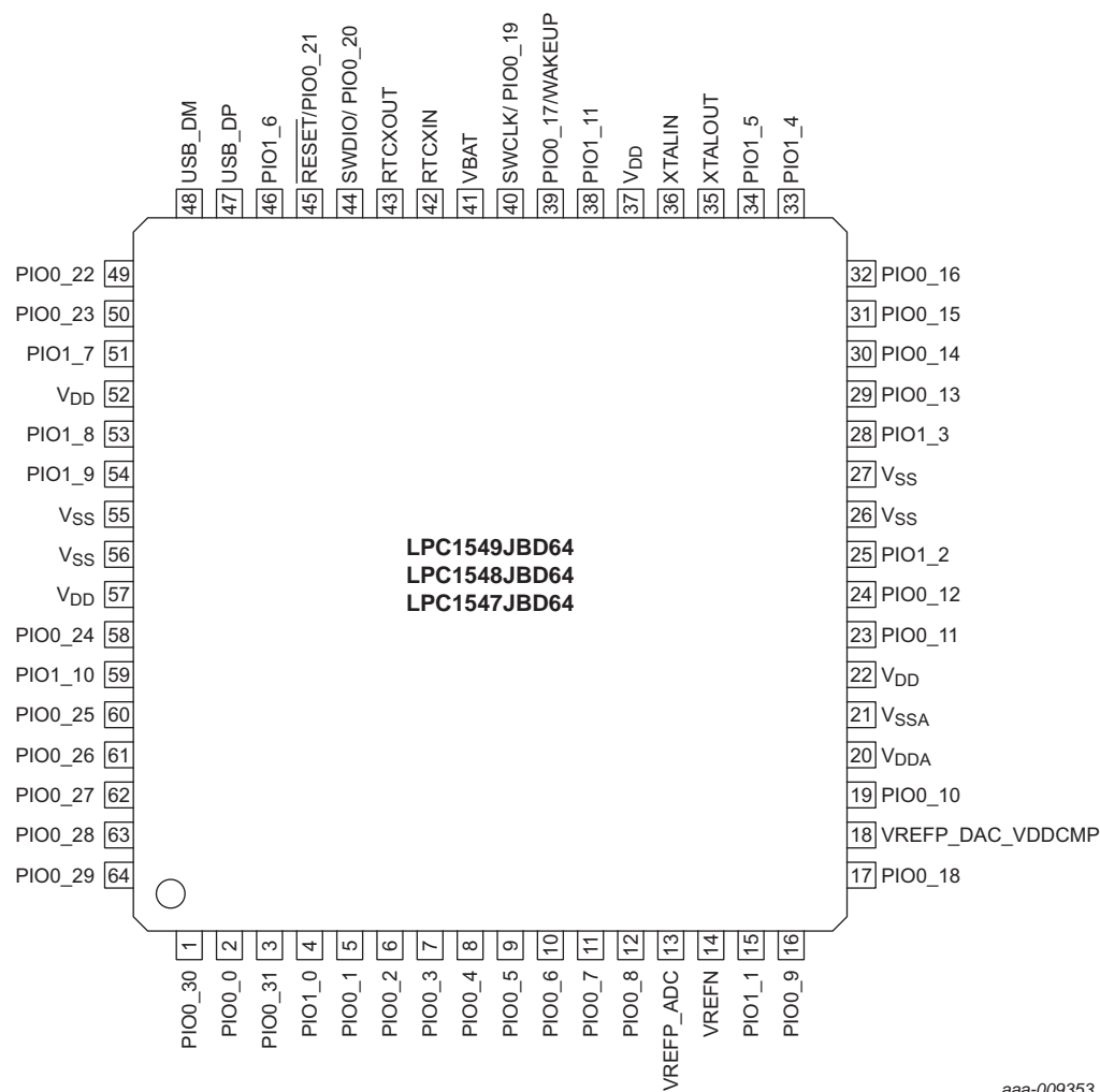
Fig 6. LQFP64 pin configuration (with USB)
