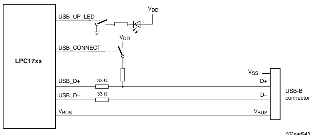
Fig 34. USB device port configuration
