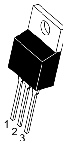
TO-220AB CASE 221A-07 STYLE 4
