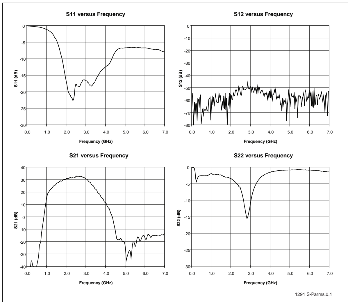
Figure 3: S-Parameters
