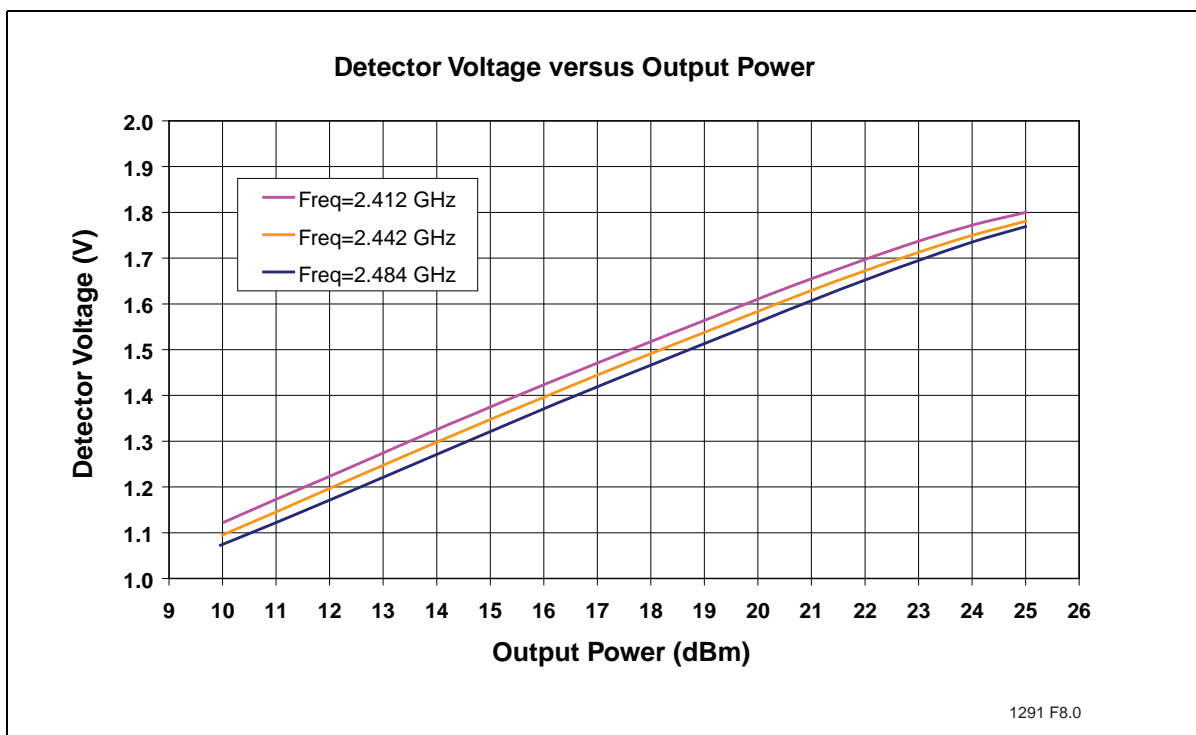
Figure 8: Detector Characteristic versus Output Power
