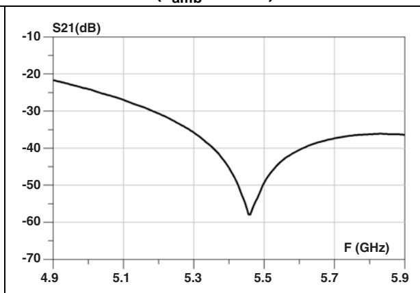
Figure 5. 2 G attenuation in 5 G band ( T_{amb} = 25\text{ }^{\circ}\text{C} )
