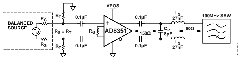
Figure 35. Example of Differential SAW Filter Interface ( f_c = 190 MHz)
