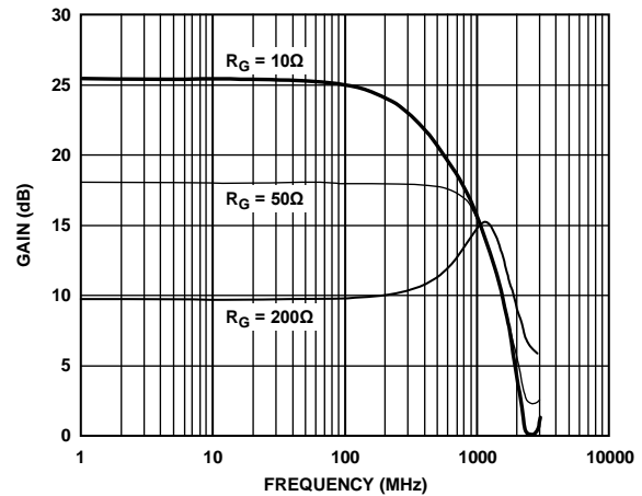
Figure 7. Gain vs. Frequency for a 1 k \Omega Differential Load ( A_V = 10\text{ dB} , 18\text{ dB} , and 26\text{ dB} )
