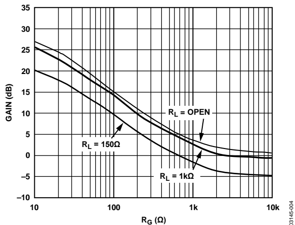
Figure 5. Gain vs. Gain Resistor, R_G ( f = 100\text{ MHz} , R_L = 150\text{ }\Omega , 1\text{ k}\Omega , and Open)
