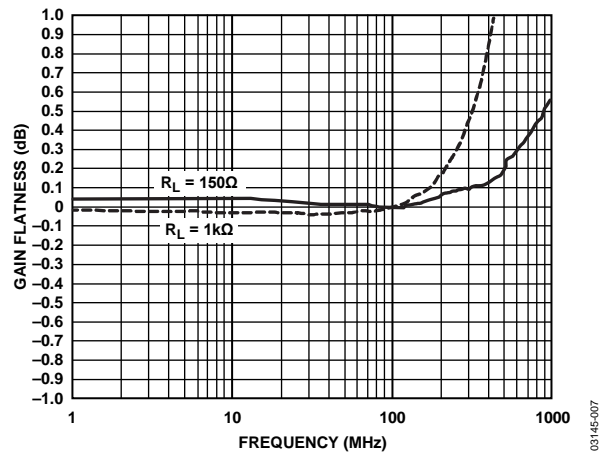
Figure 8. Gain Flatness vs. Frequency ( R_L = 150\text{ }\Omega and 1\text{ k}\Omega , A_V = 10\text{ dB} )
