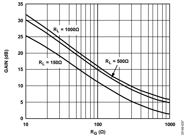
Figure 38. Gain Selection
