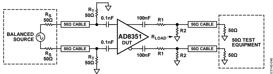
Figure 47. Test Circuit
