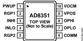
Figure 2. MSOP Pin Configuration
