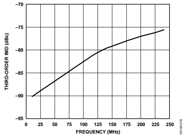
Figure 19. Third-Order Intermodulation Distortion vs. Frequency for a 2 V p-p Composite Signal into R_L = 1\ \text{k}\Omega ( A_V = 10\ \text{dB} , at 5 V Supplies)
