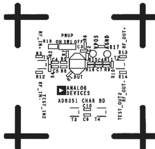
Figure 49. Component Side Silkscreen
