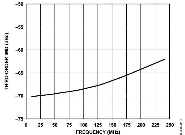
Figure 20. Third-Order Intermodulation Distortion vs. Frequency for a 2 V p-p Composite Signal into R_L = 150\ \Omega ( A_V = 10\ \text{dB} , at 5 V Supplies)
