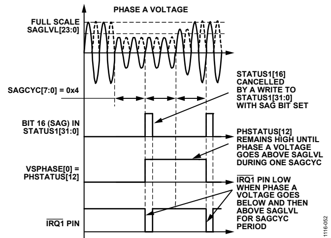
Figure 60. Sag Detection: SAGCFG Bit in ACCMODE Register Set to 1
