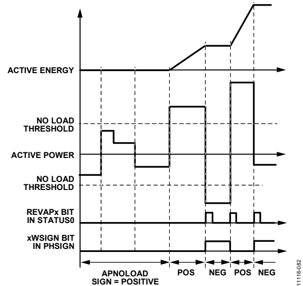
Figure 88. Active Power Positive Only Accumulation Mode
