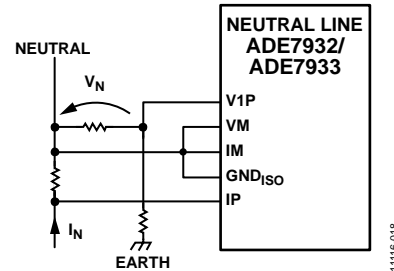
Figure 102. Neutral Line and Neutral to Earth Voltage Monitoring with the ADE7933/ADE7932
