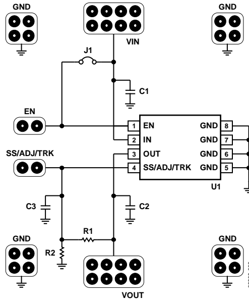
Figure 2. Evaluation Board Schematic
