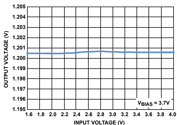
FIGURE 10. V_{\text{IN}} LINE REGULATION
