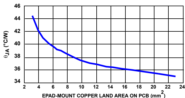
FIGURE 37. 3mmx3mm-10 PIN DFN ON 4-LAYER PCB WITH THERMAL VIAS θ JA vs EPAD-MOUNT COPPER LAND AREA ON PCB
