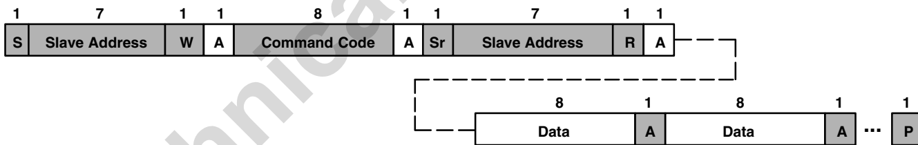
Figure 10. I 2 C Protocols
