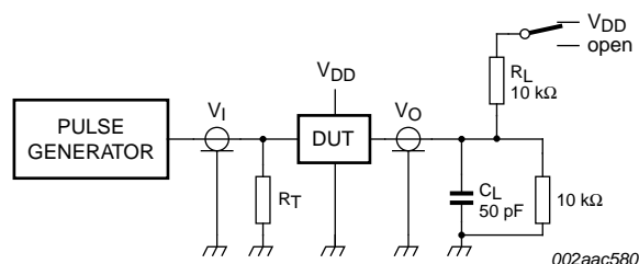
Fig 15. Test circuitry for enable/disable times, SDOOUT ( t_{\text{en}}(\text{SDOOUT}) and t_{\text{dis}}(\text{SDOOUT}) )
