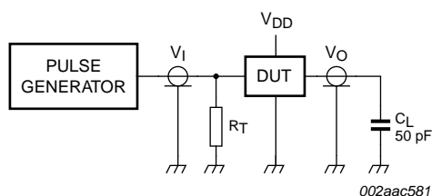
Fig 16. Test circuitry for switching times, SDOOUT ( t_v(\text{SDOOUT}) )
