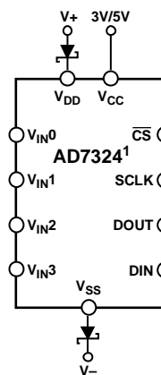
1 ADDITIONAL PINS OMITTED FOR CLARITY.
