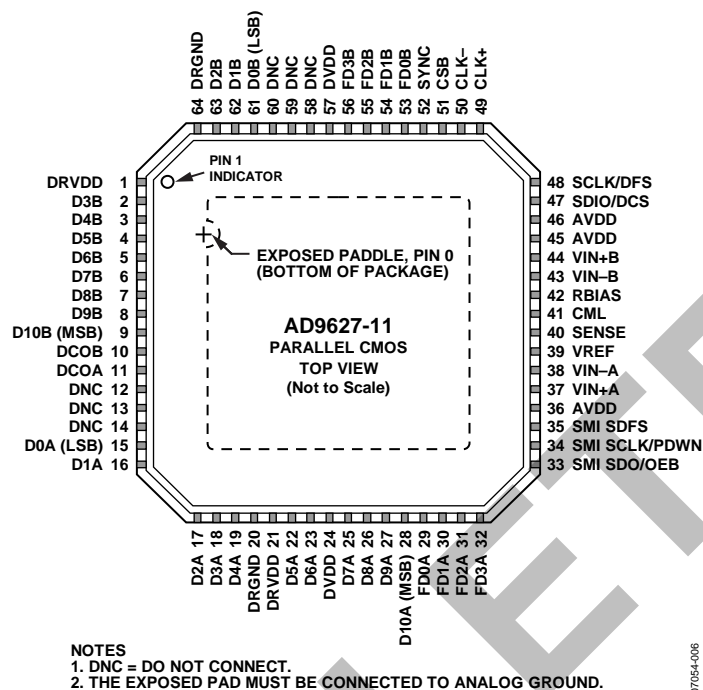
Figure 6. LFCSP Parallel CMOS Pin Configuration (Top View)
