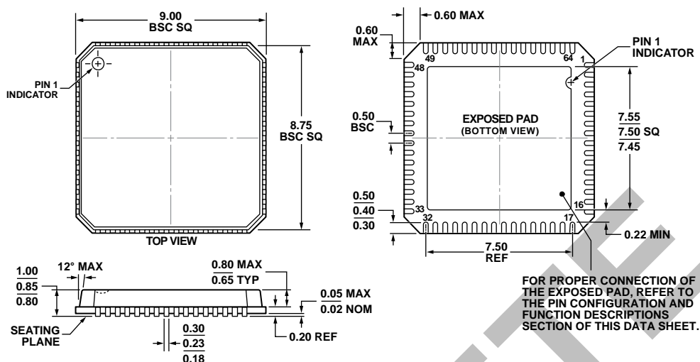
Figure 91. 64-Lead Lead Frame Chip Scale Package [LFCSP_VQ] 9 mm x 9 mm Body, Very Thin Quad (CP-64-6) Dimensions shown in millimeters
