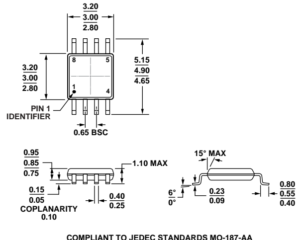
Figure 34. 8-Lead Mini Small Outline Package [MSOP] (RM-8)
