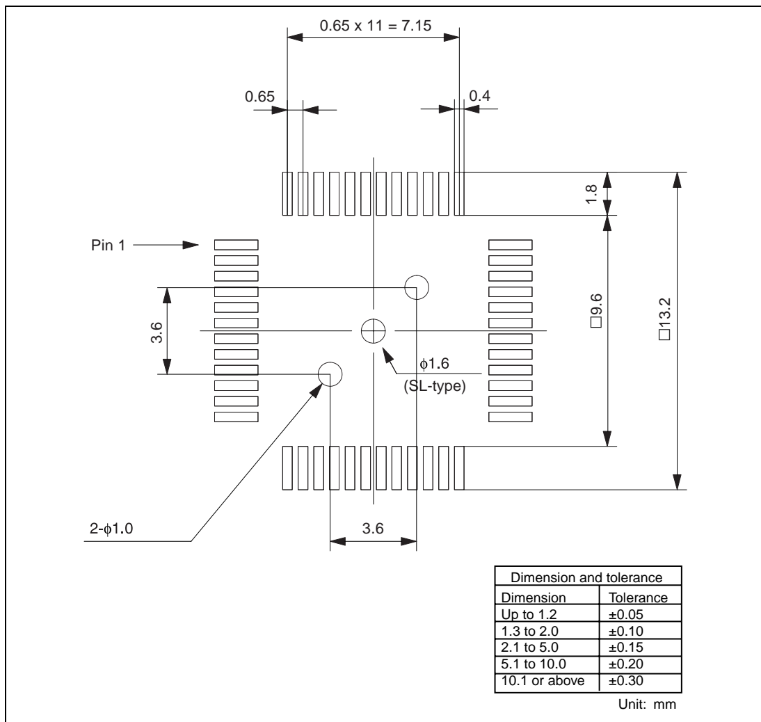
Figure 4 Recommended Dimensions for Mount Pad
