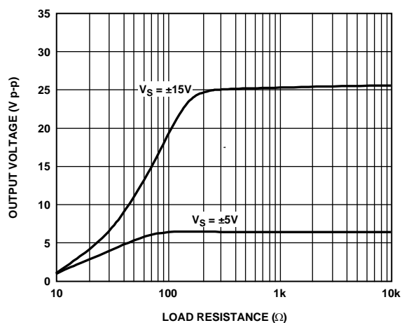
Figure 8. Output Voltage Swing vs. Resistive Load
