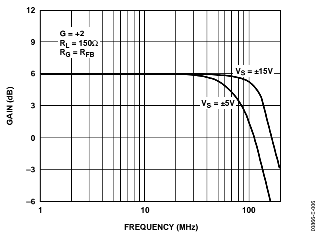
Figure 6. Frequency Response
