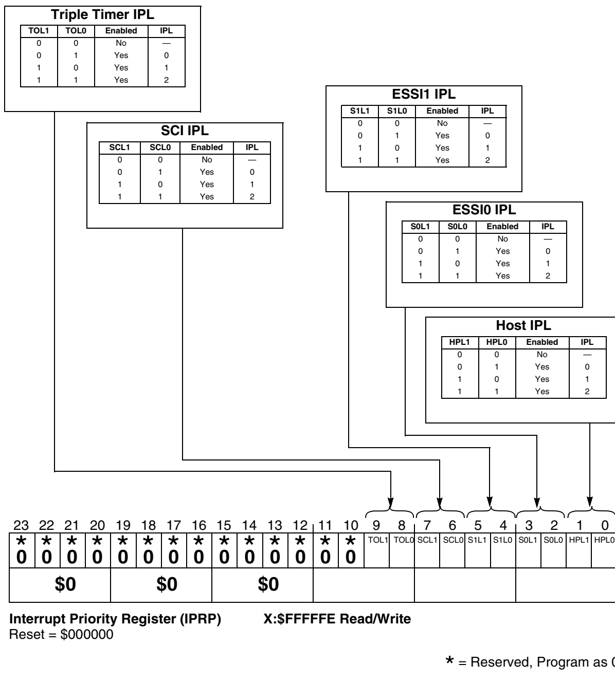
Figure B-3. Interrupt Priority Register-Peripherals (IPRP)
