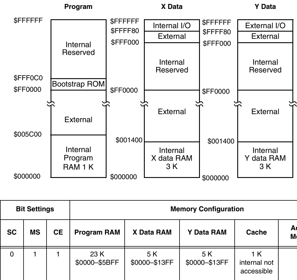
Figure 3-4. Switched Program RAM and Instruction Cache Enabled (0, 1, 1)
