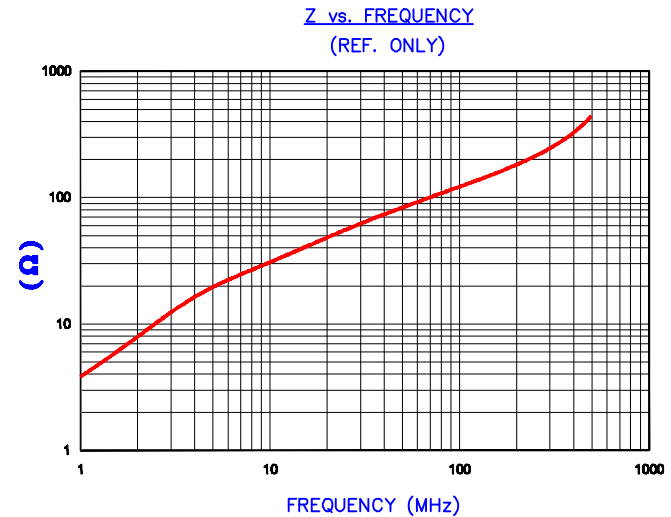
AGILENT E4991A Impedance/Material Analyzer HP 16092A-Test Fixture, REF # 3903
