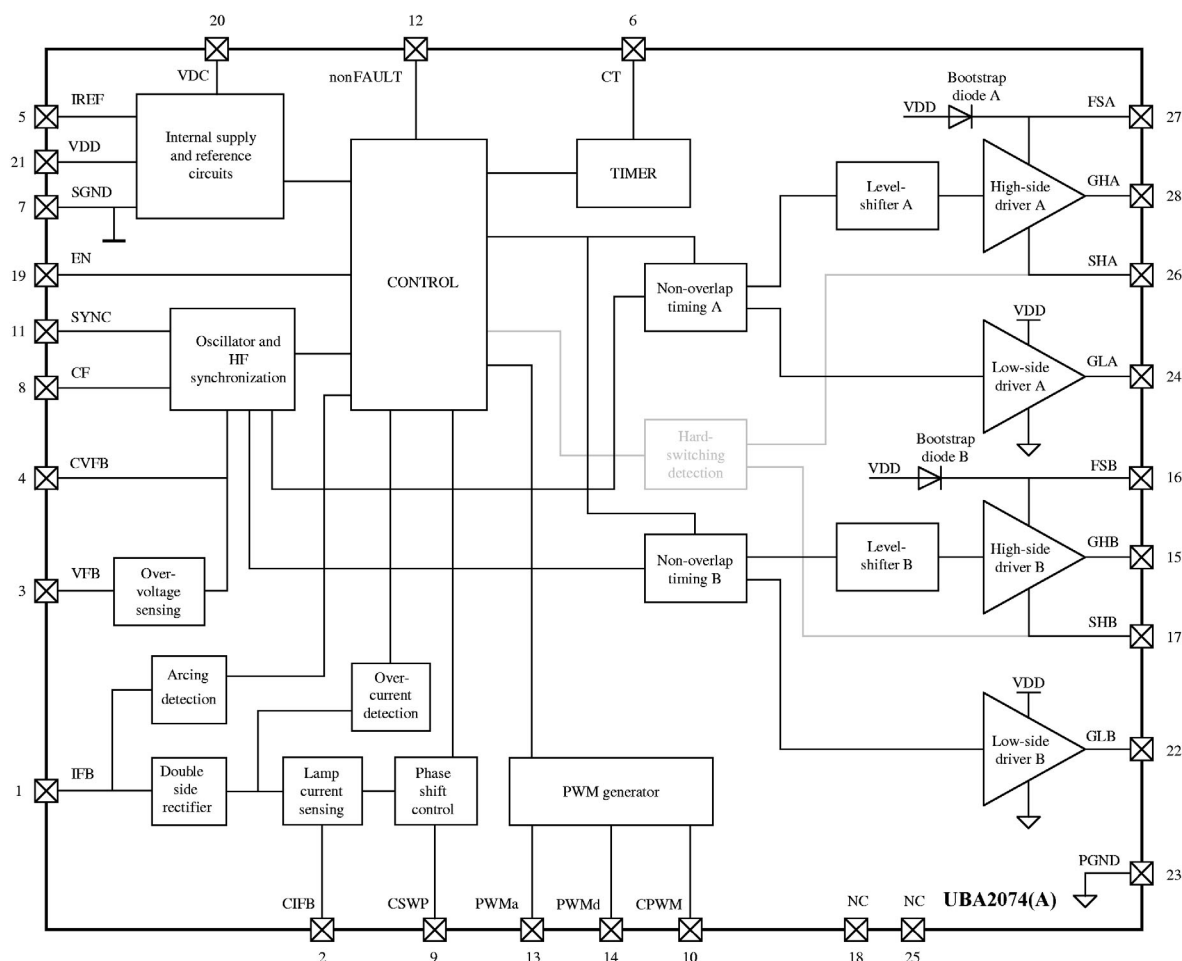
Fig 1. Block diagram UBA2074(A) (Shaded circuit not present in the UBA2074A).
