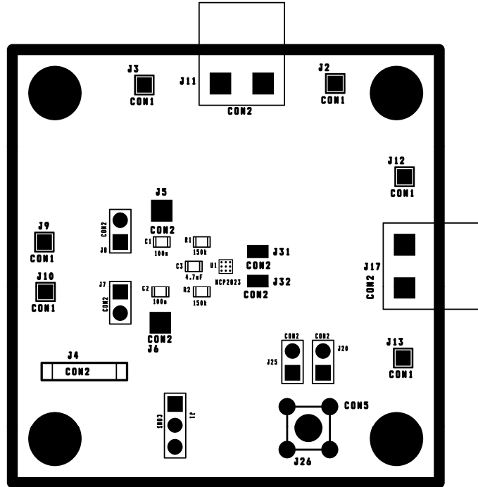
Figure 10. Assembly Layer TOP
