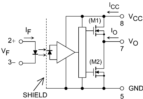
Fig. 5.1 Internal Circuit
