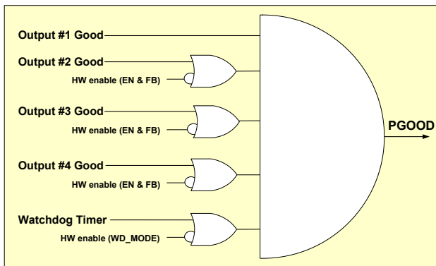
Figure 17 - Hardware Mode PGOOD Generation
