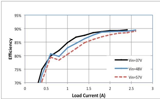
Figure 2. AF, V_{out1} = 5V Efficiency Using PoE13P-15L Transformer
