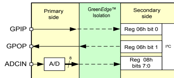
Figure 22 - GPIO and ADC Pin Mapping
