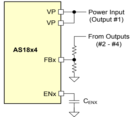
Figure 15 - HW Mode Output(s) Hardware Disabled
