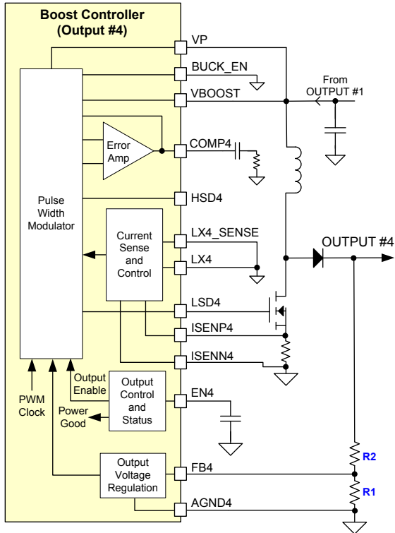
Figure 12 - Power Output #4 Block Diagram - BOOST
