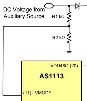
Figure 5 – AS1113 LVMODE Connection
