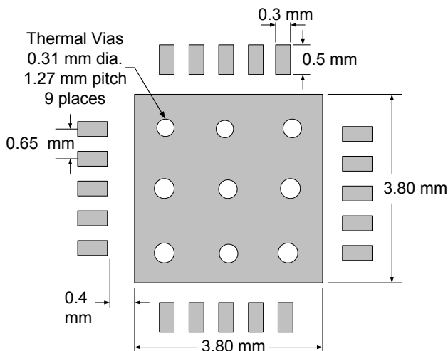
Figure 7 – AS1113 PCB Footprint
