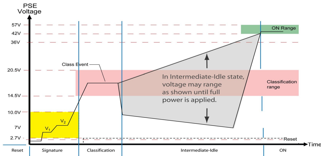
Figure 6. Representative Power-On waveform
