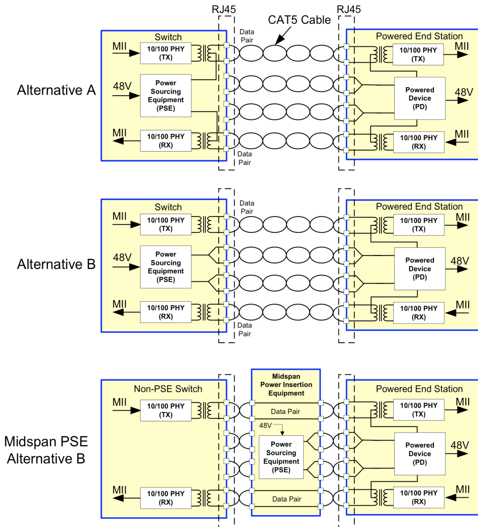
Figure 3. IEEE® Std. 802.3af-2003 Power Feeding Schemes for 10/100 Systems
