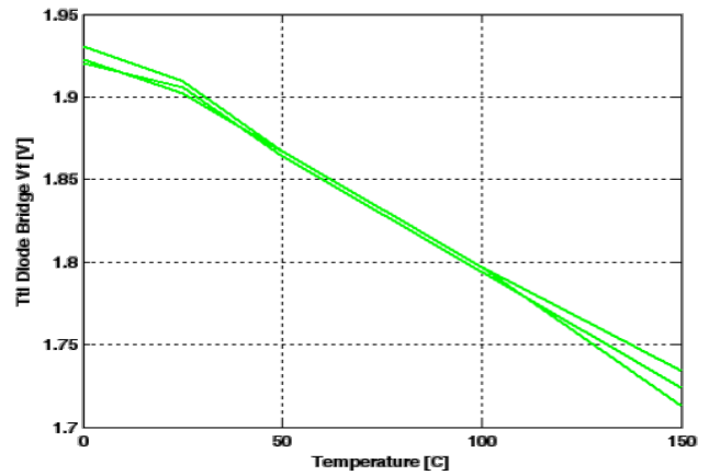
Full Load Diode Bridge V_F vs. Junction Temperature
