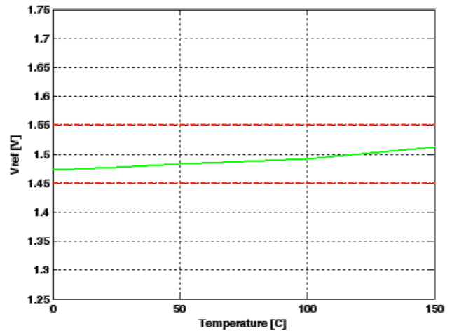
Error Amplifier Ref. Voltage vs. Junction Temperature
