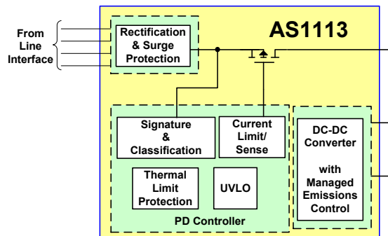
Figure 4 – Top-Level Block Diagram of the AS1113
