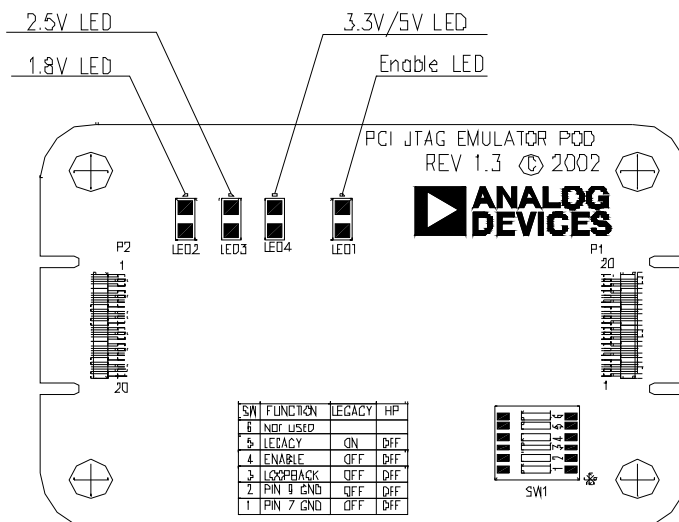
Figure 2-1. Pod LEDs
