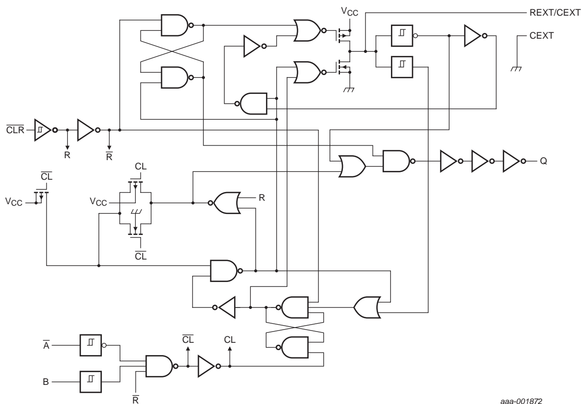
Fig 2. Logic diagram
