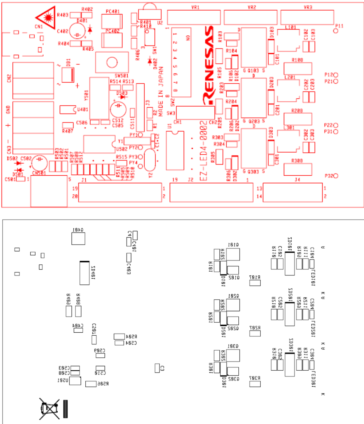
Figure 41: Top and Bottom Silkscreen
