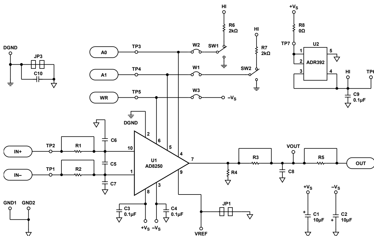
Figure 1. Schematic
