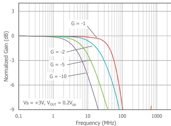
Inverting Freq. Resp.
