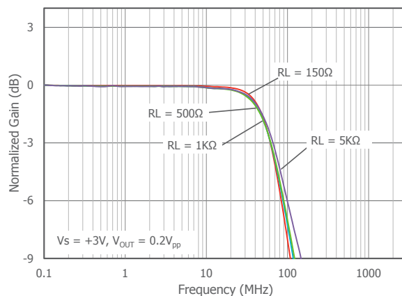
Freq. Resp. vs RL
