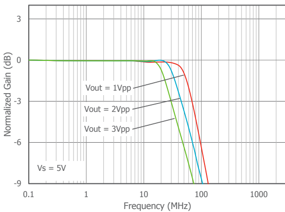
Large Signal Freq. Resp.
