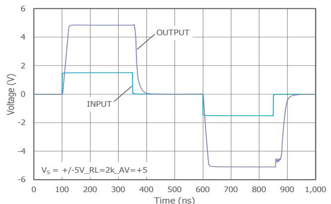
Figure 5: Overdrive Recovery
