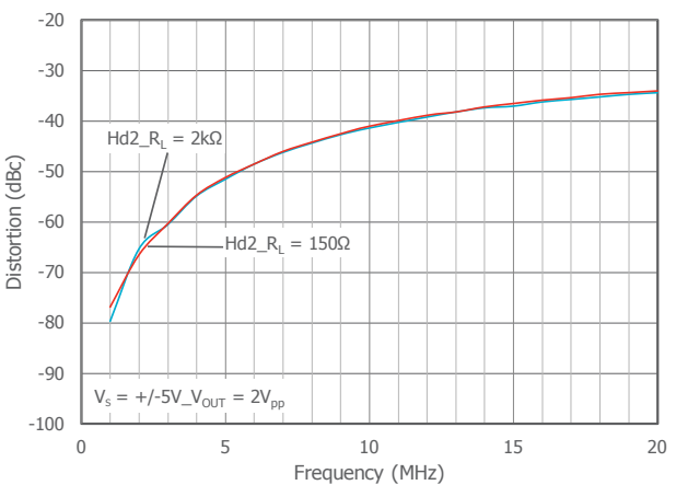
2nd Harmonic Distortion Vs RL over Freq.
