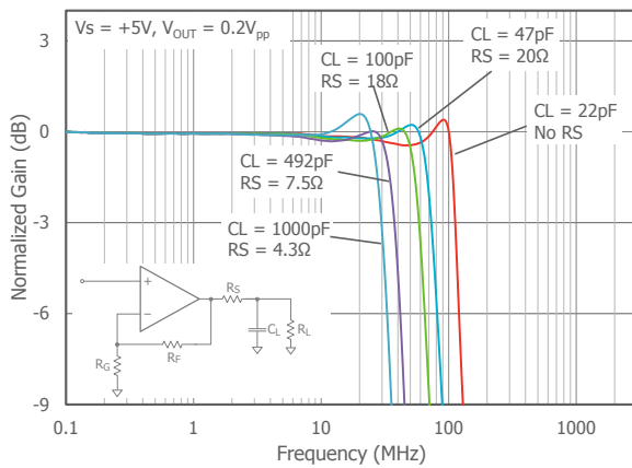
Freq. Resp. vs CL
