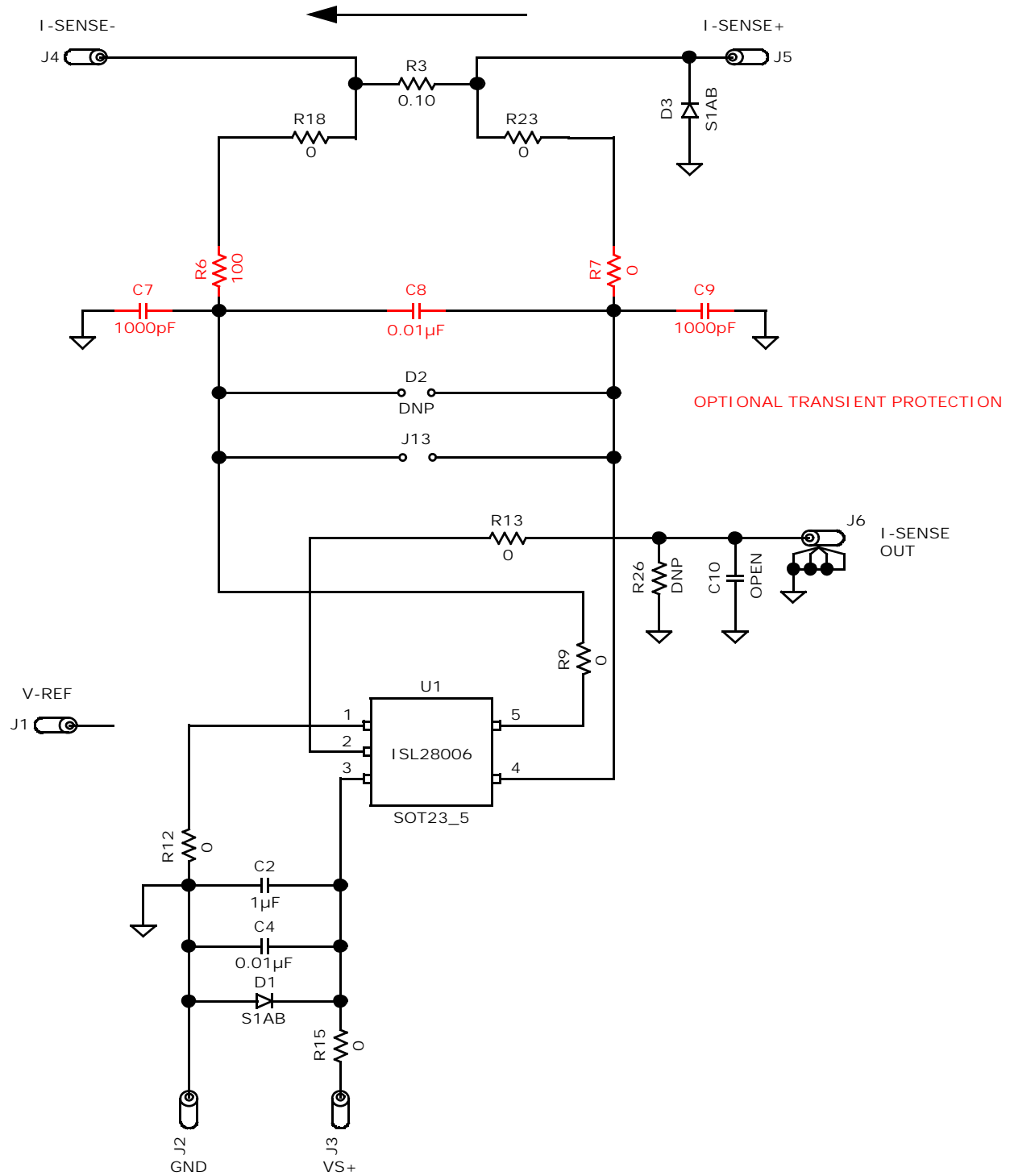
FIGURE 1. SIMPLIFIED ICL2800XEVAL1Z SCHEMATIC DIAGRAM FOR FIXED GAIN PARTS
