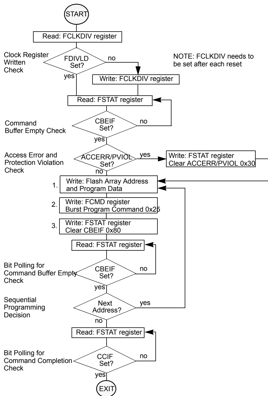
Figure 88. Example Burst Program Command Flow
