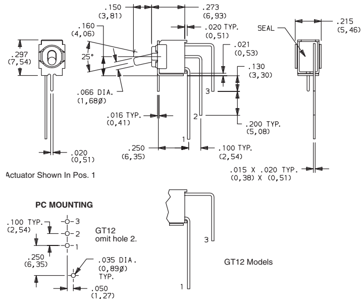
PART NUMBER SWITCH FUNCTION POS.1 POS. 2 POS. 3 GT11MAVBE GT13MAVBE ON ON NONE OFF ON ON Conn. Terms. 2-3 OPEN 2-1 Schematic SPDT GT12MAVBE OFF NONE ON Conn. Terms. OPEN N/A 3-1 Schematic SPST
