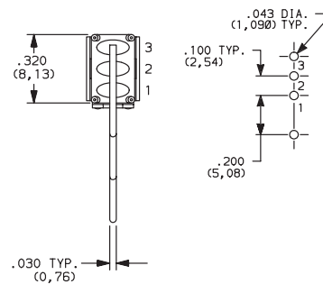
ET01SD1AV2BE Vertical Actuation SPDT
