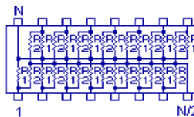
DUAL TERMINATOR [Schematic 5]
