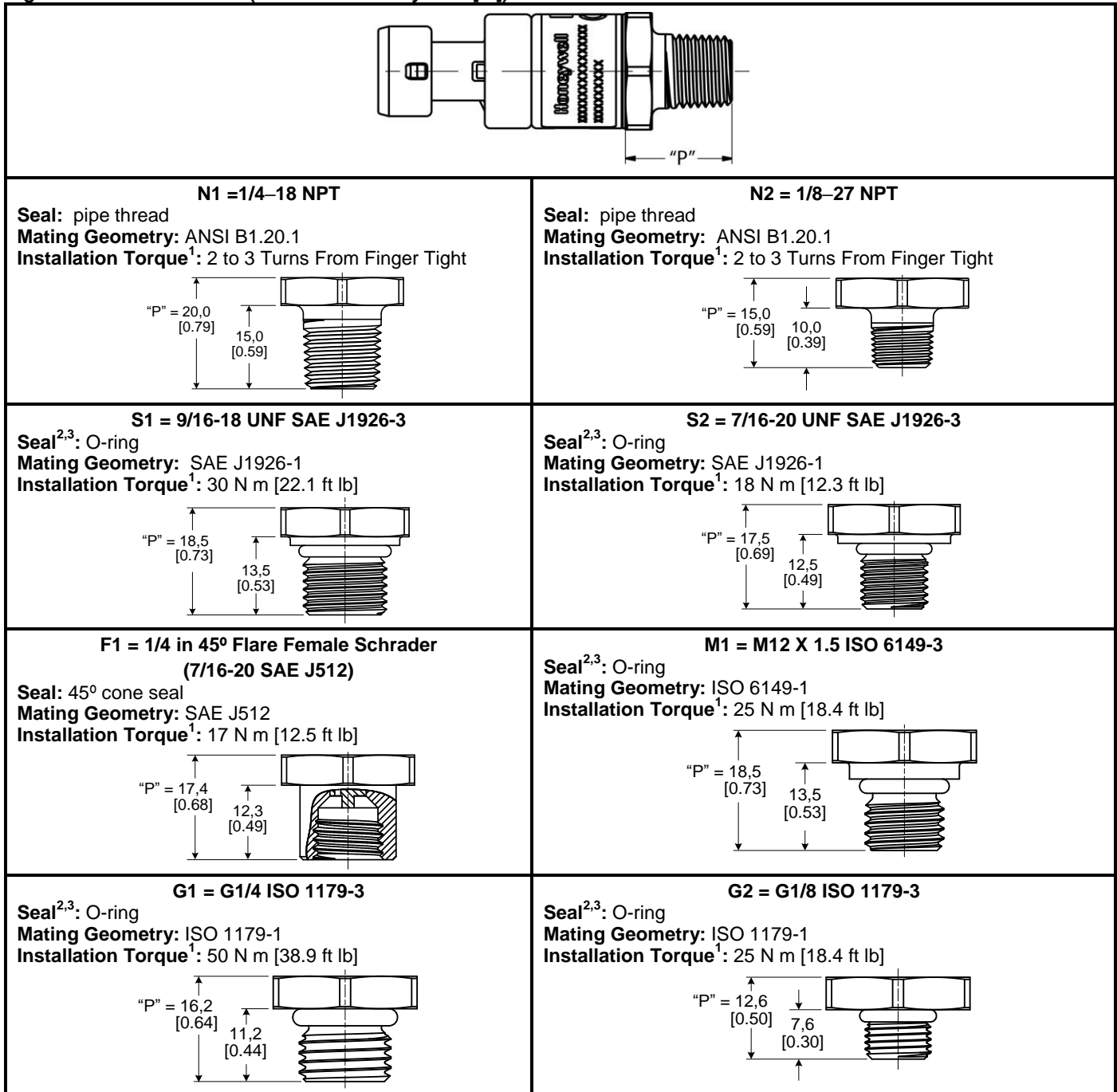
Figure 8. Port Dimensions (For reference only: mm/[in])
