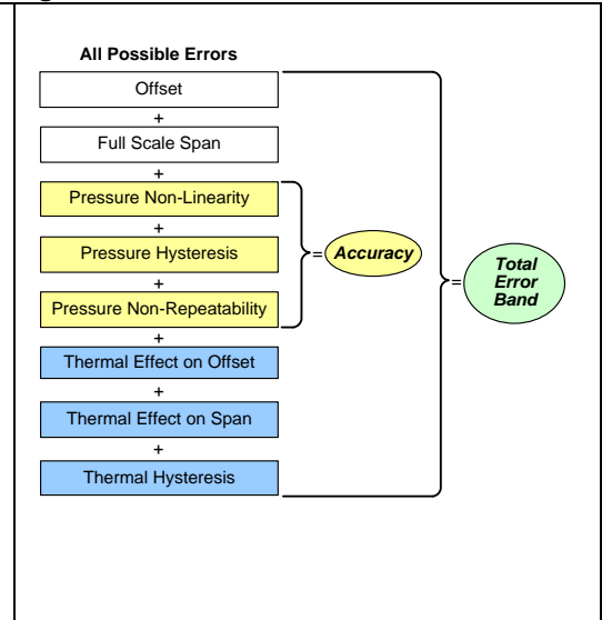
Figure 4. Total Error Band
