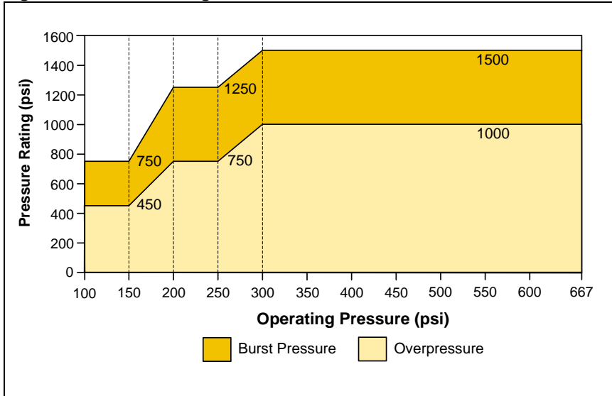
Figure 3. Pressure Rating Curve
