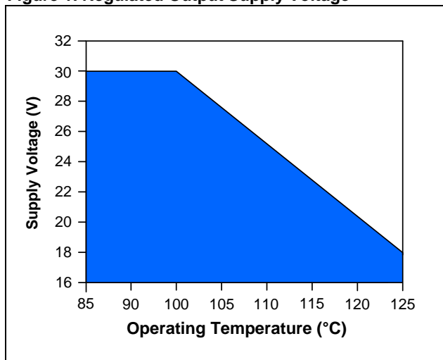
Figure 1. Regulated Output Supply Voltage
