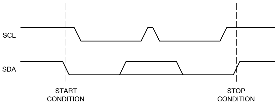
Figure 2. START/STOP Conditions
