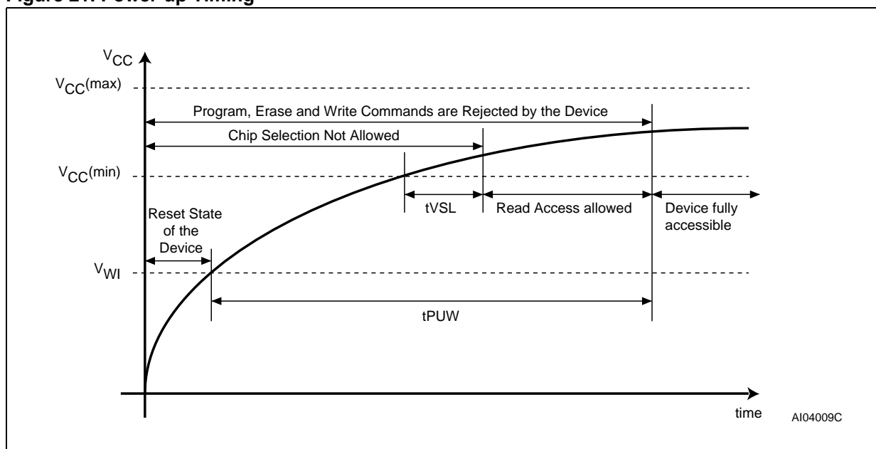
Figure 21. Power-up Timing
