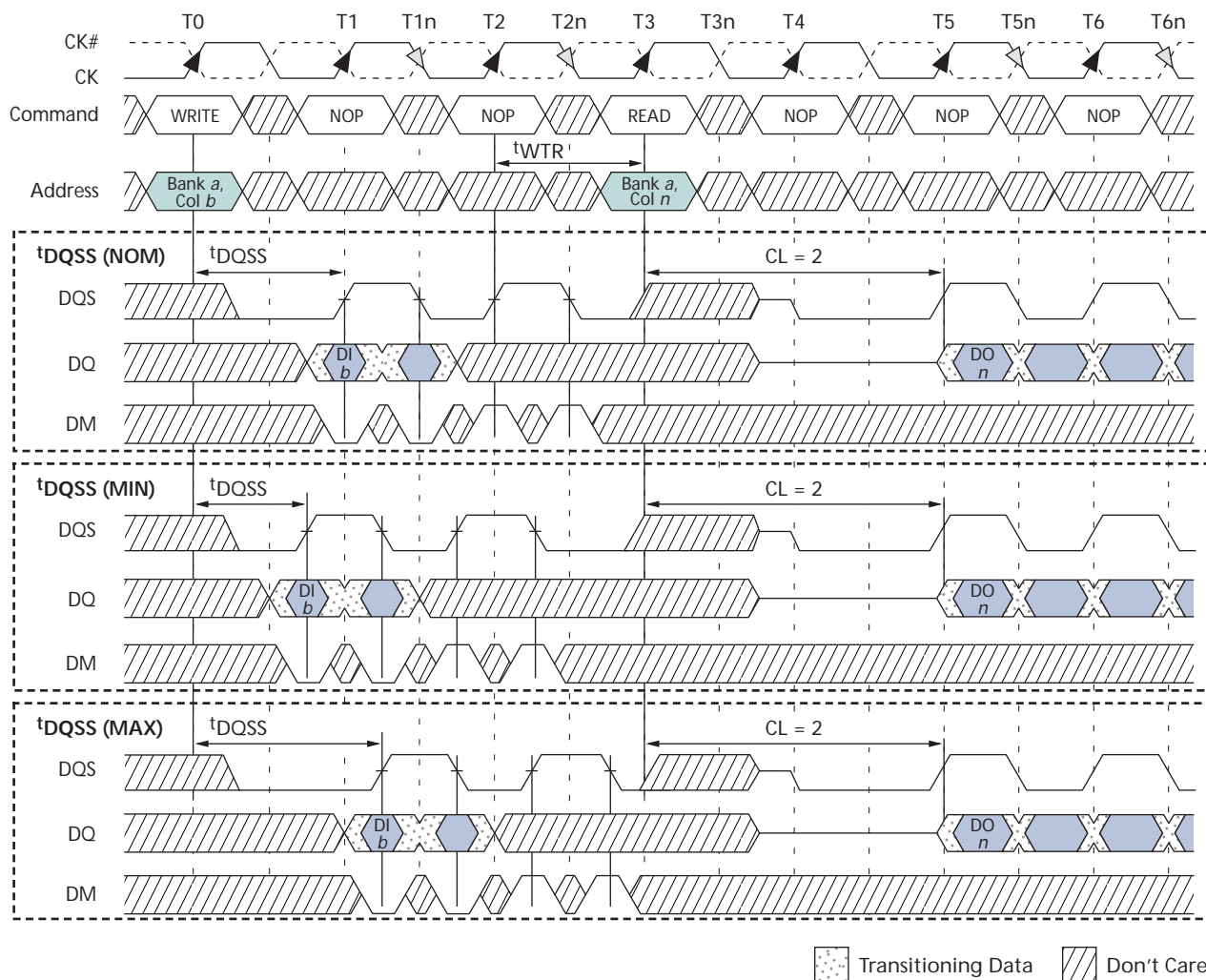
Figure 43: WRITE-to-READ – Interrupting
