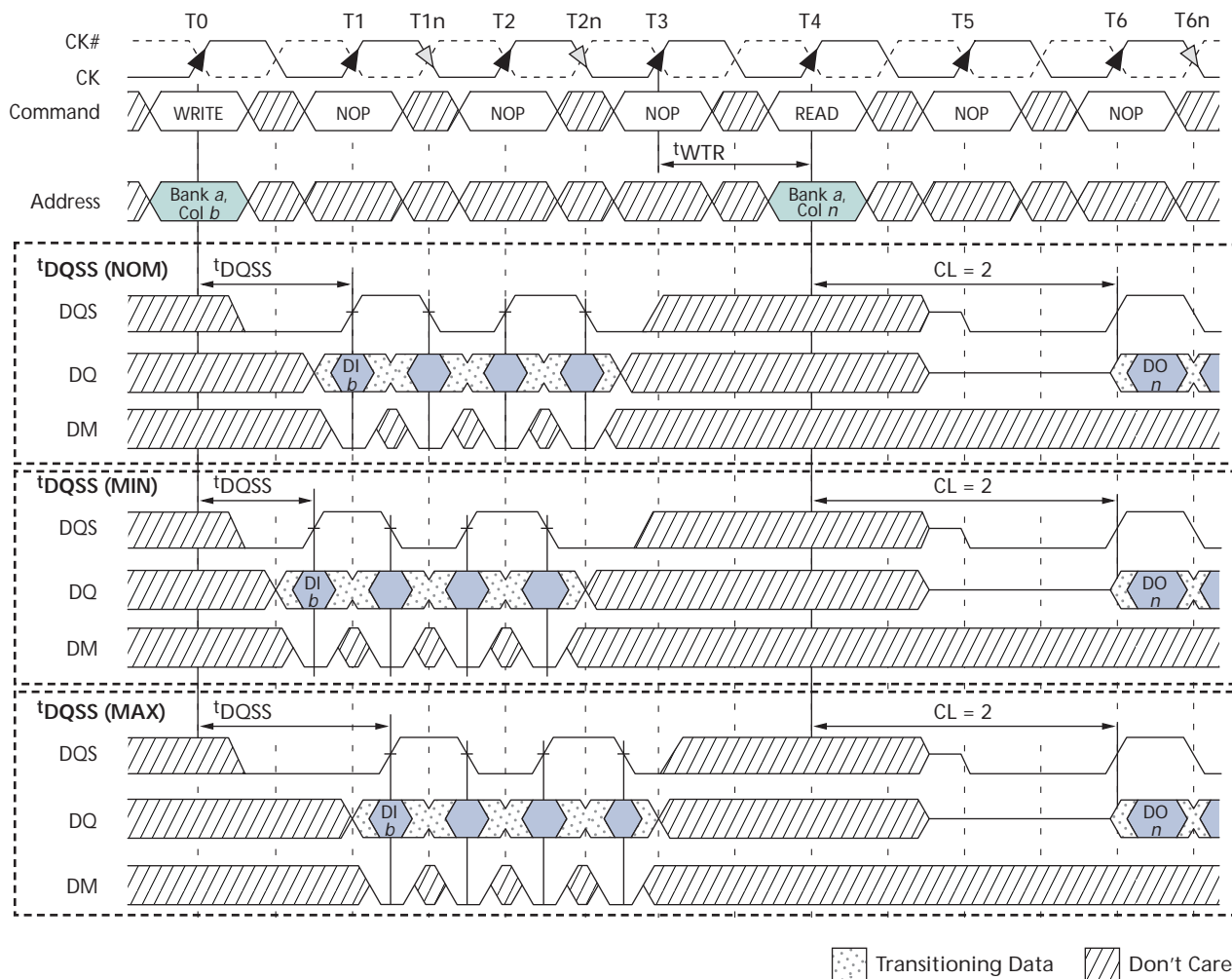
Figure 42: WRITE-to-READ – Uninterrupting
