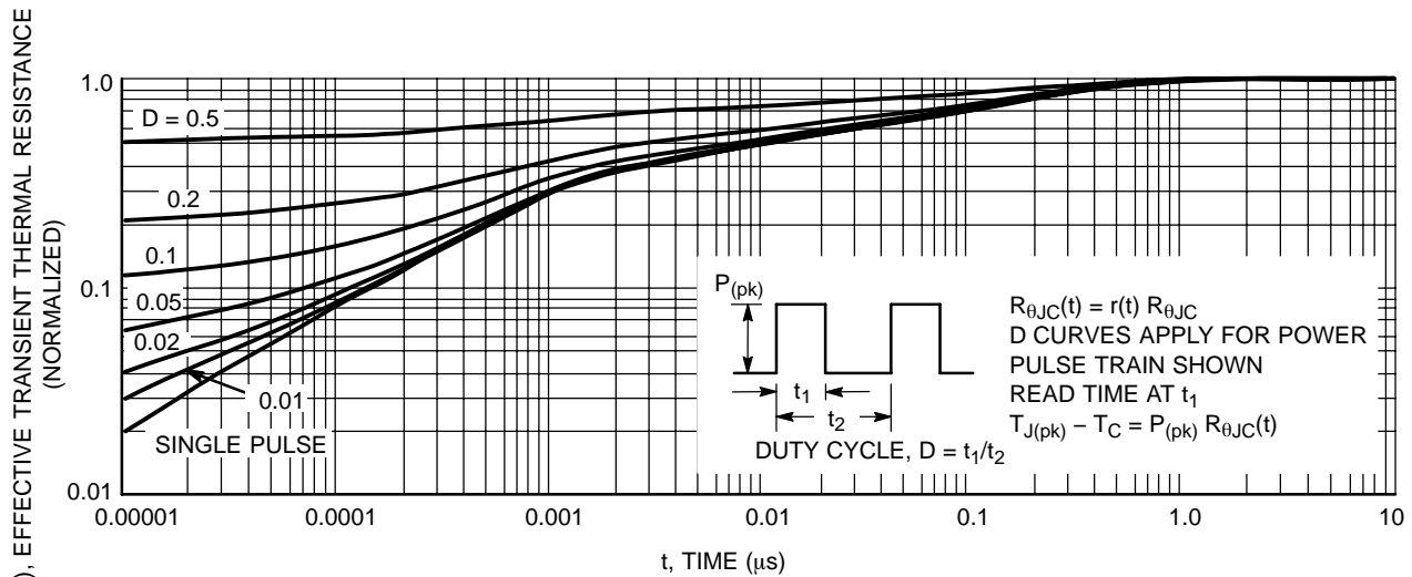
Figure 13. Thermal Response
