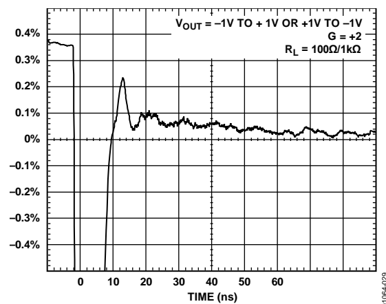
Figure 27. Settling Time
