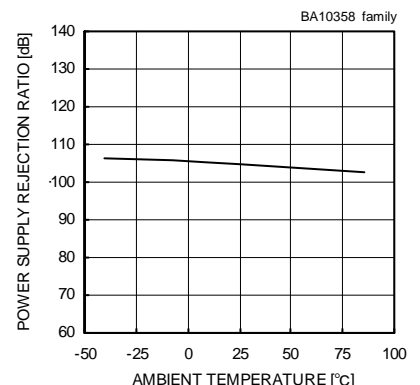
Fig. 24 Power Supply Rejection Ratio - Ambient Temperature
