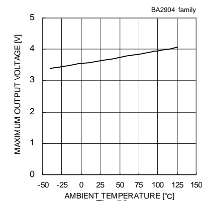
Fig. 53 Maximum Output Voltage - Ambient Temperature ( V_{CC}=5[V] , R_L=2[k\Omega] )
