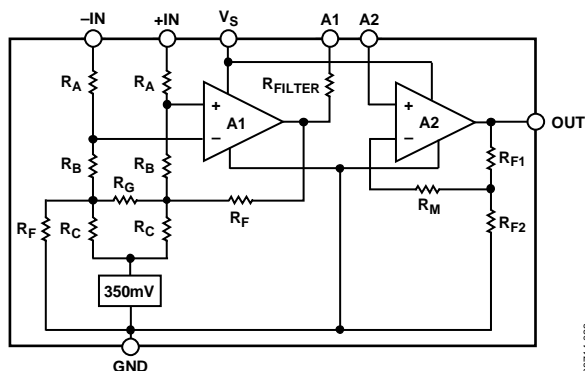
Figure 24. Simplified Schematic
