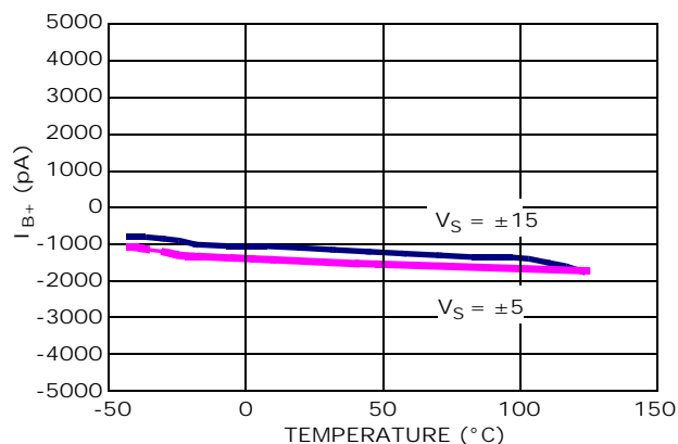
FIGURE 9. I_{B+} vs TEMPERATURE vs SUPPLY VOLTAGE
