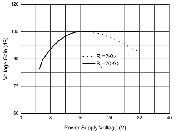
Figure 7. Voltage Gain
