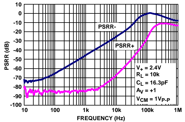
FIGURE 10. PSRR vs FREQUENCY, V_+ = 2.4V , V_- = \pm 1.2V
