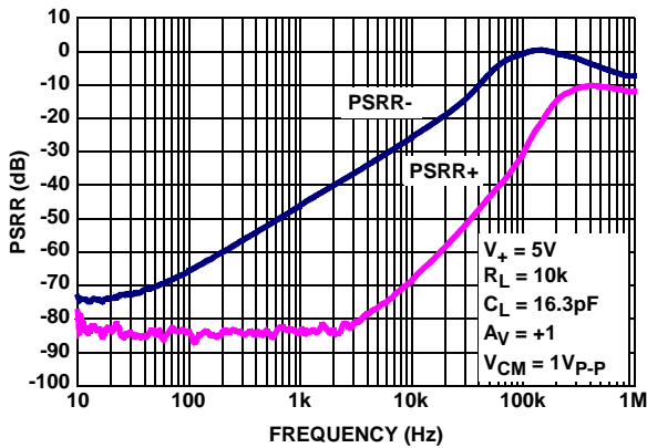
FIGURE 11. PSRR vs FREQUENCY, V_+ = 5V , V_- = \pm 2.5V
