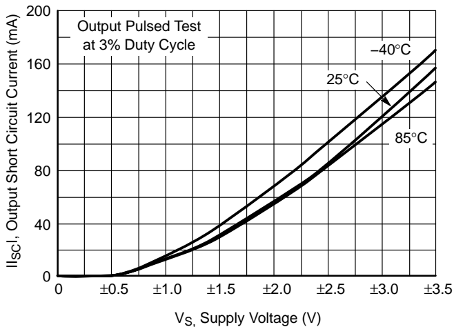
Figure 12. Output Short Circuit Sourcing Current vs. Supply Voltage
