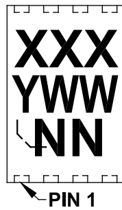
8-Lead UDFN (2x3x0.5 mm)
